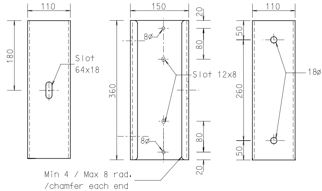
BLOCKOUT PIECE – W BEAM (P002)
