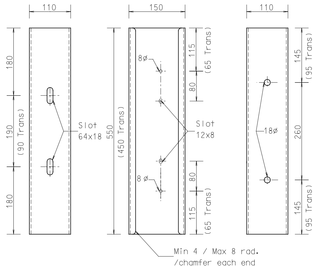
BLOCKOUT PIECE – THRIE BEAM (P004) – TRANSITION (P005)
