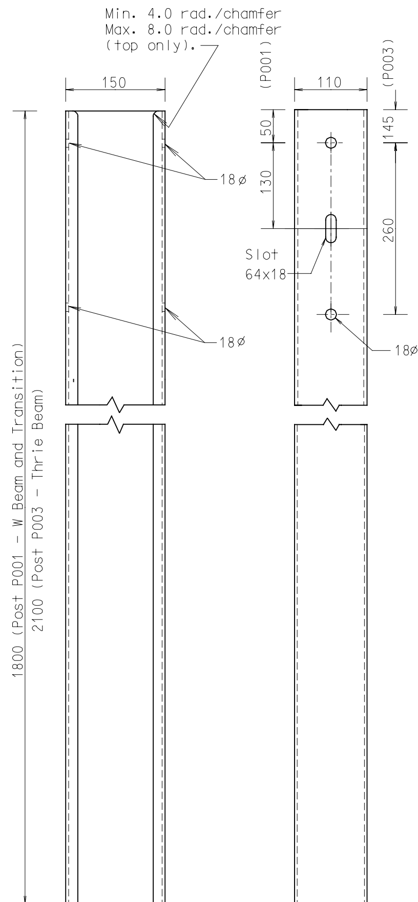
POST - W BEAM (P001) - THRIE (P003)
