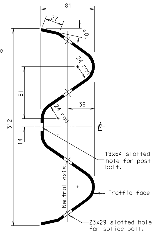
SECTION THROUGH RAIL / STIFFENER (Position of Slotted Holes Shown).
