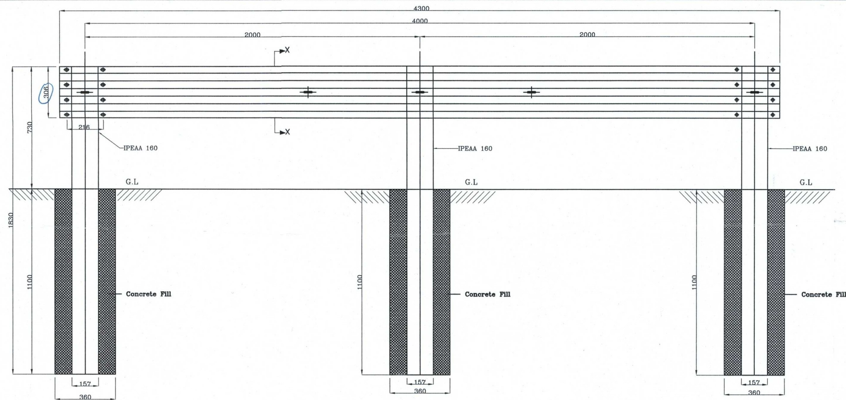
SINGLE SIDED GUARDRAIL FRONT VIEW
