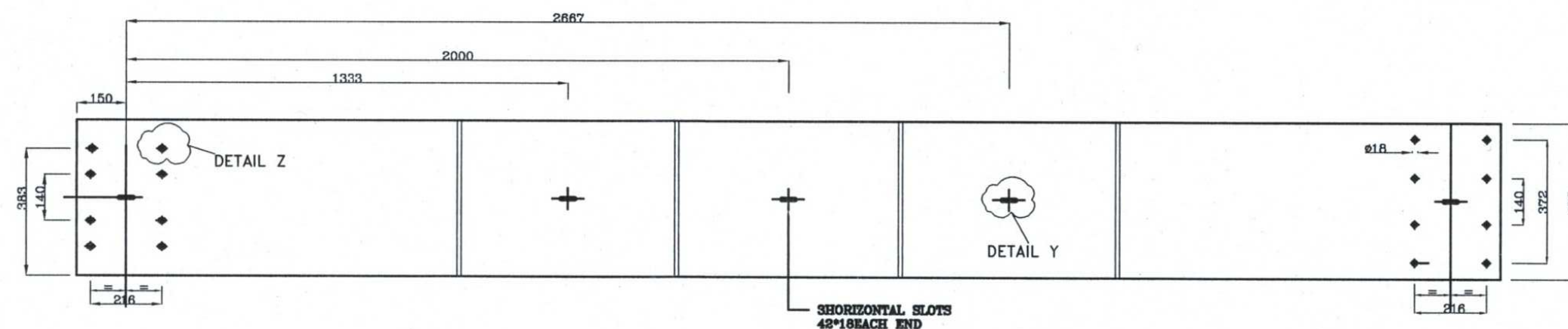
STANDARD BEAM-BEFORE CORRUGATION
