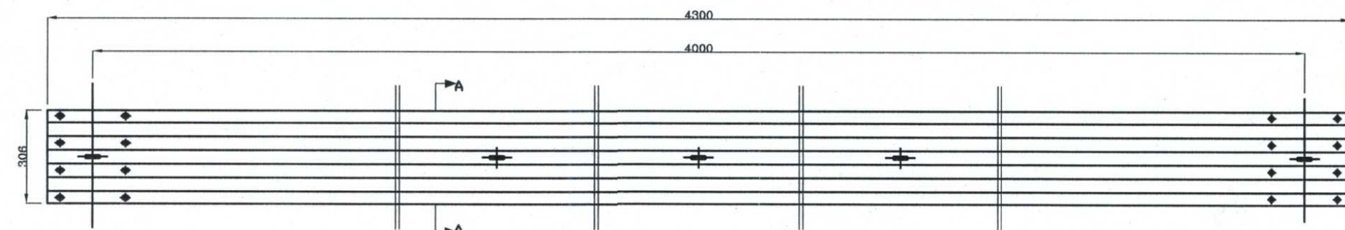
SINGLE SIDE GUARDRAIL-FRONT VIEW
