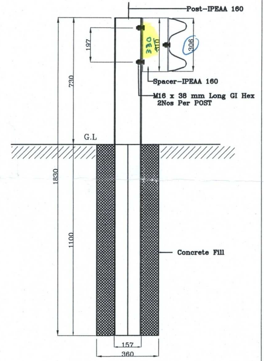
SECTION X-X
