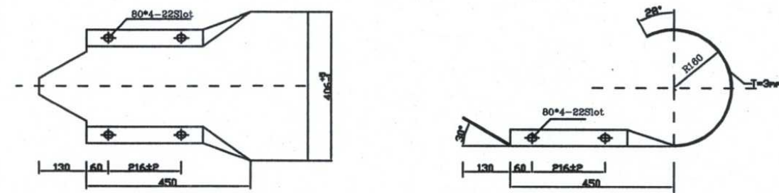
W BEAM END SECTION DETAIL
