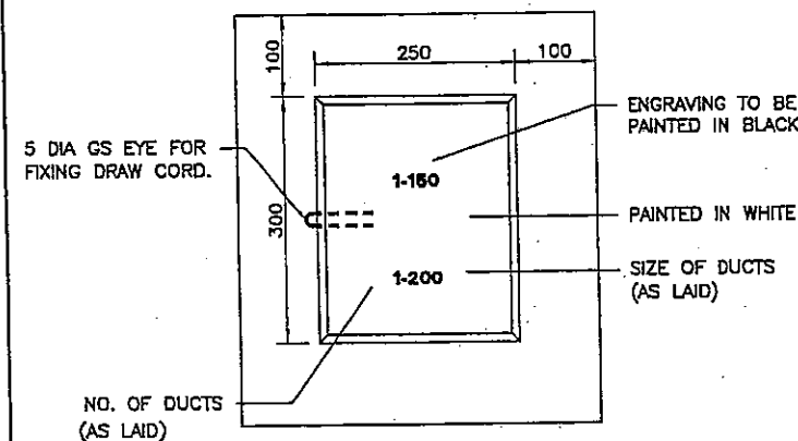
PLAN PRECAST DUCT MARKER
