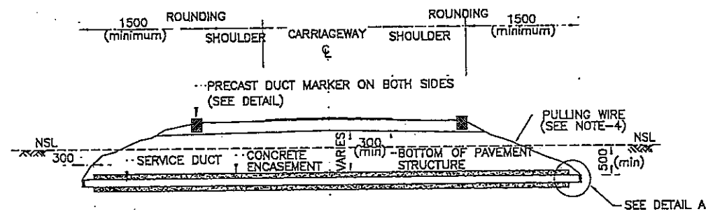
TYPICAL CROSS SECTION OF SERVICE DUCTS ACROSS RAMPS
