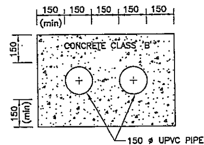
SECTION A-A (FUTURE DUCTS FOR ELECTRICAL CABLES)
