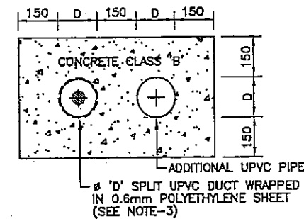
DUCT FOR PROTECTION OF EXISTING SERVICES
