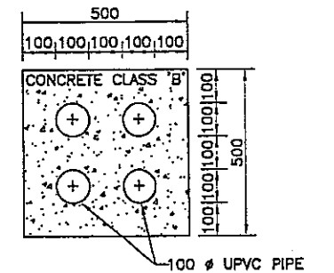
SECTION B-B (FUTURE DUCTS FOR TELEPHONE CABLES 4 WAY)
