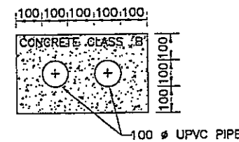
SECTION B-B (FUTURE DUCTS FOR TELEPHONE CABLES TWO WAY)
