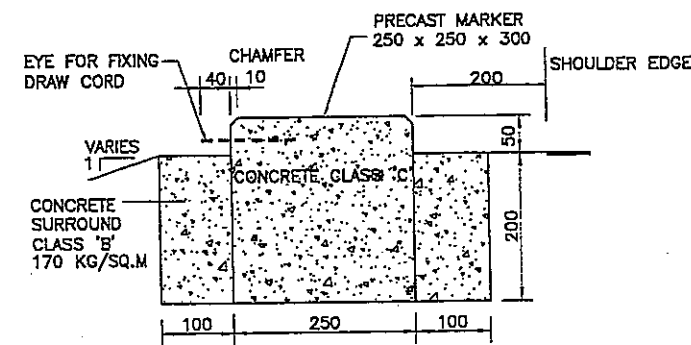
ELEVATION PRECAST DUCT MARKER
