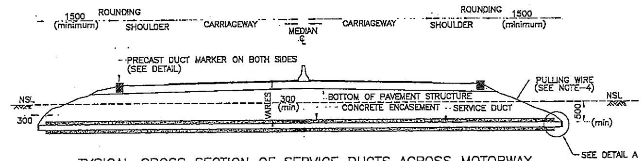
TYPICAL CROSS SECTION OF SERVICE DUCTS ACROSS MOTORWAY
