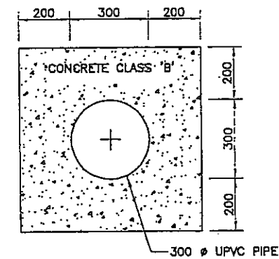
SECTION C-C (FUTURE DUCTS FOR WATER LINES)
