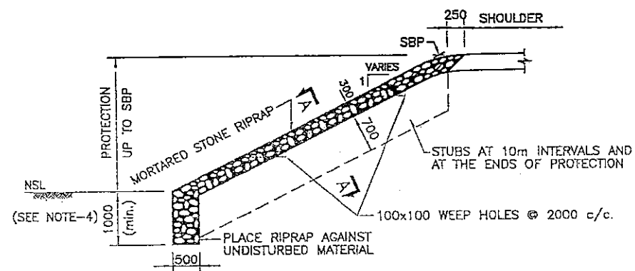
GROUTED STONE RIPRAP PROTECTION (EP-1)
