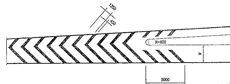
DETAIL "C"
