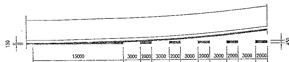
DETAIL "A"
