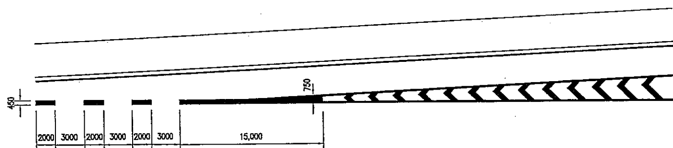
DETAIL "B"
