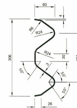
SECTION A - A Not to Scale
