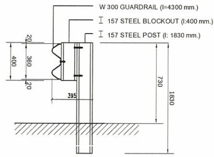
TYPICAL GUARDRAIL CROSS SECTION Not to Scale
