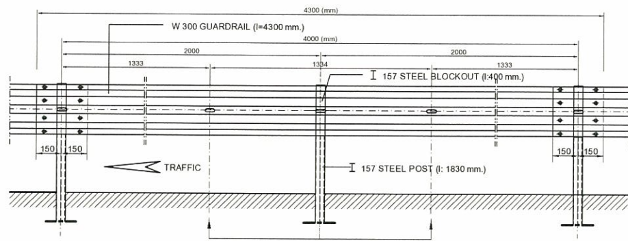
SINGLE SIDE GUARDRAIL FRONT VIEW Not to Scale
