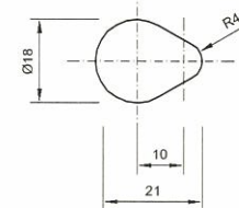
DETAIL X Not to Scale
