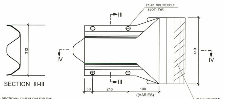
W BEAM END SECTION DETAIL Not to Scale
