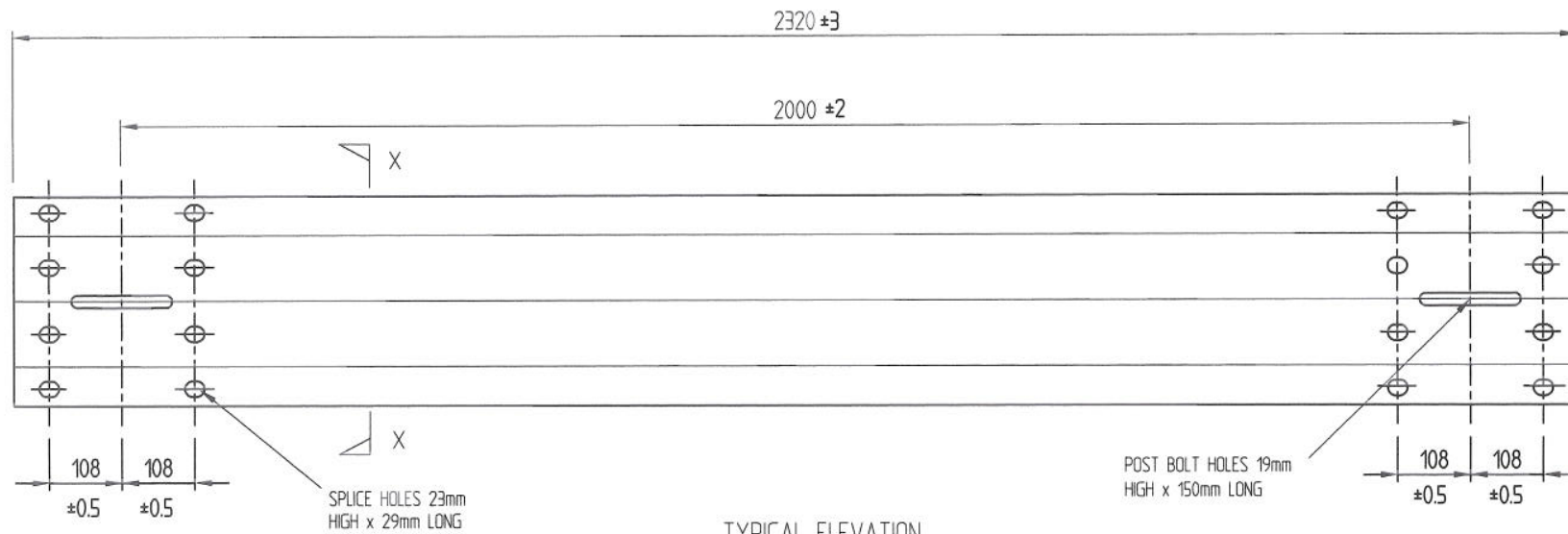
TYPICAL ELEVATION
